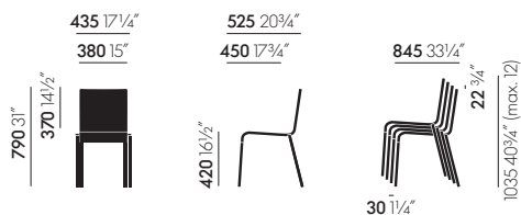
.03, stacking
